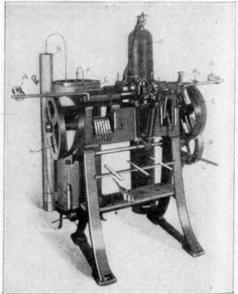
Fig. 16. Automatic Machine for welding Lead-in Wires
